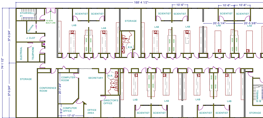
whitley MB-4240-2 SECOND FLOOR AREA 12173 sq ft
